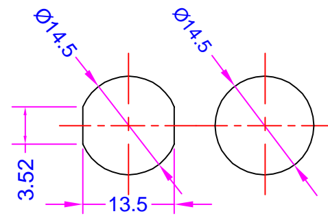
Mounting Hole
