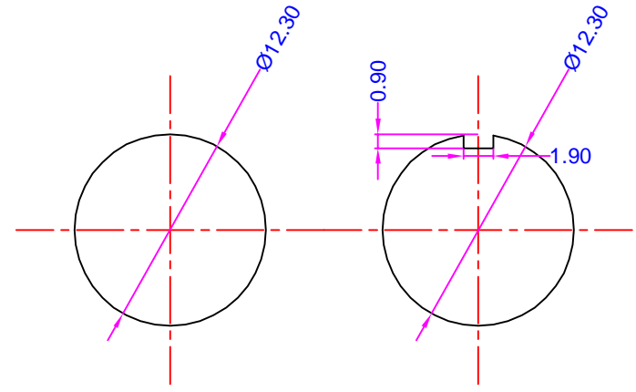
Mounting Hole
